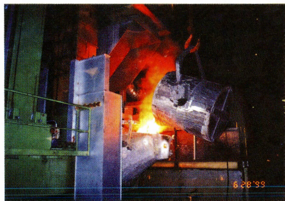
図6 受湯状態 Fig.6 Pouring to GF converter from transfer ladle
