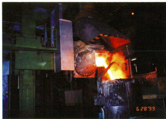
図8 出湯状態 Fig.8 Tapping from GF converter to transfer ladle
