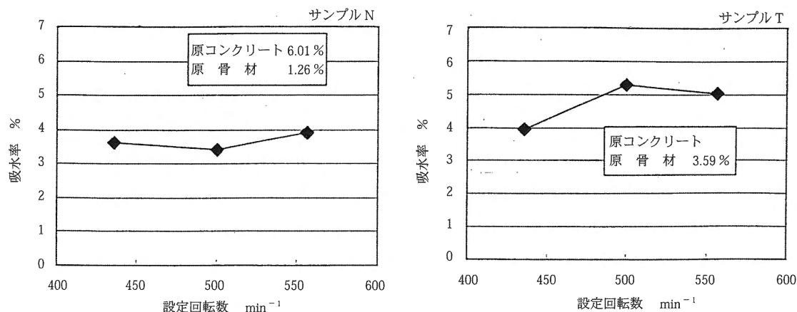
図8 吸水率 Fig. 8 Water absorption
