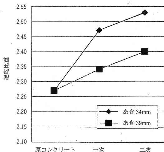
図4 絶乾比重
