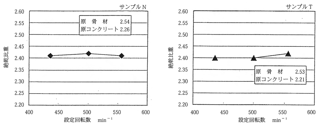
図7 絶対比重 Fig. 7 Specific gravity in absolute dry condition
