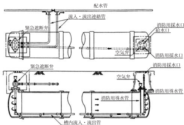
図2 集中Ⅱ型耐震性貯水槽構造 Fig. 2 Typical structure of aseismatic water storage tank of combination model II
