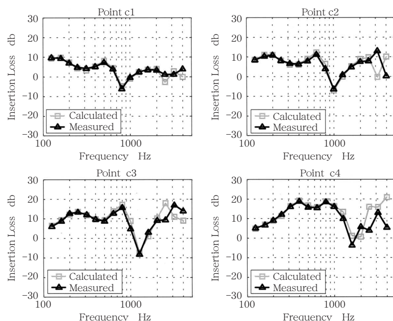
図7 c列における低層遮音壁の実験と計算による挿入損失 Fig. 7 Insertion loss of low noise barrier by measured and analysis on the line of receiving points c-series
