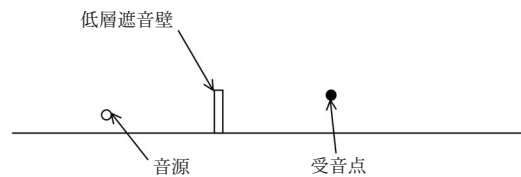
図1(b) 音源、遮音壁、受音点の配置図 Fig. 1(b) Geometry the line source, low noise barrier, and receivers
