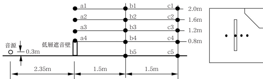
図4 実験および計算における配置 Fig. 4 Geometry of sound source, receiving points and low noise barrier on experiment and analysis
