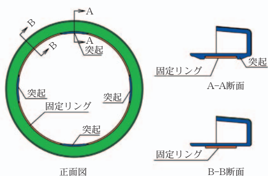
図2 NS形用防食ゴム形状 Fig. 2 Shape of corrosion prevention rubber for NS-type joint
