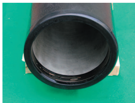
図1 防食ゴムの取付け状況(K形) Fig. 1 Installation state of corrosion prevention K-type rubber
