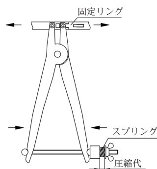
図17 拡張機構 Fig. 17 Expansion mechanism of the tool
