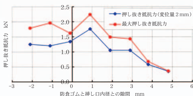
図13 押し抜き抵抗確認試験結果 Fig. 13 Performance test result of resistance against pushing force
