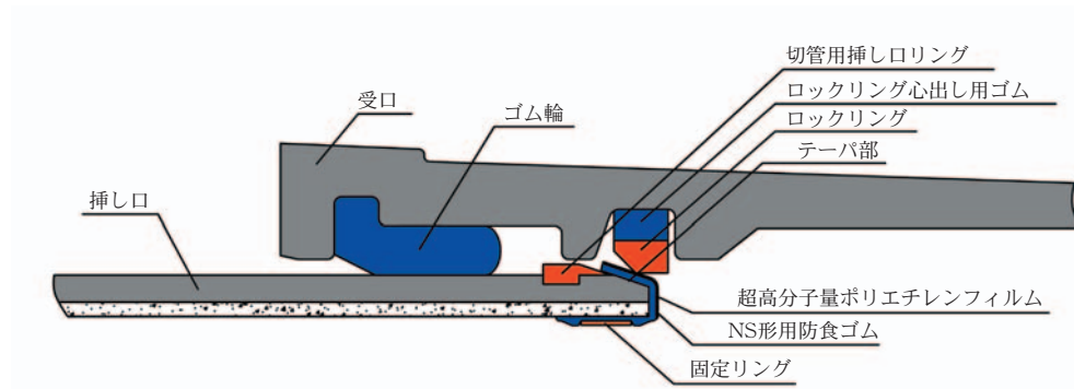
図10 接合試験時の防食ゴムの状況 Fig. 10 State of corrosion prevention rubber of joint
