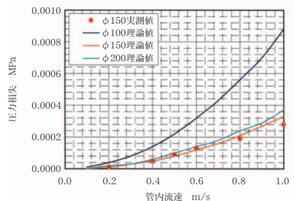
図5 損失水頭の実測値と理論値 Fig. 5 Test result in loss of head of apparatus (φ150) and calculated by theory
