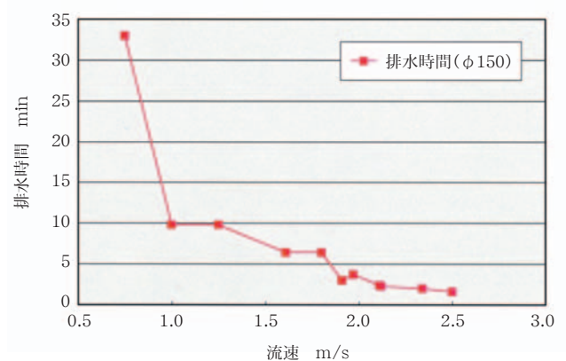
図12 砂の効率的洗管時間(分/100m) Fig. 12 Efficient cleaning time to remove (min/100m)
