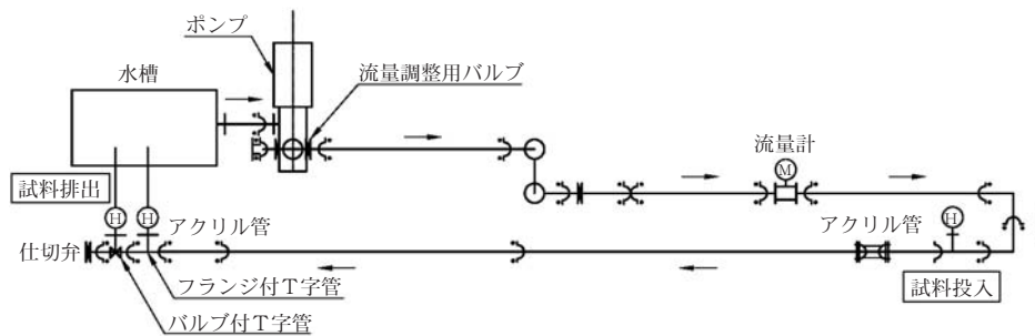
図6 排出試験管路 Fig. 6 Piping for remove performance test
