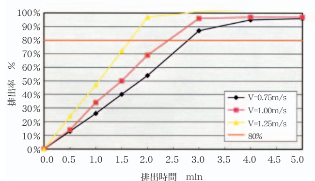
図11 排出率と排出時間の関係(塗料片) Fig. 11 Relation between the rate of removal and lapsed time (Broken pieces of a paint)
