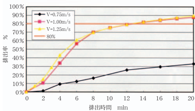
図10 排出率と排出時間の関係(砂) Fig. 10 Relation between the rate of removal and lapsed time (sand)
