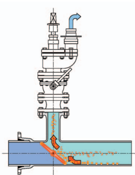
図2 洗管時の状態 Fig. 2 Valve Position on draining
