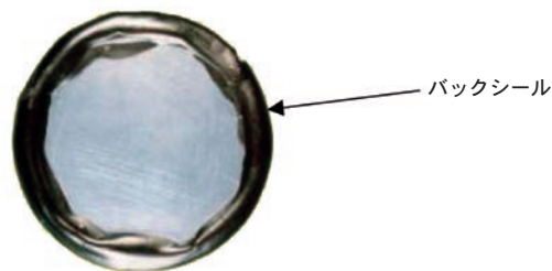
図12 溶射被膜のSST結果 (2000h後) Fig.12 SST of Mg_2Si spray coating after 2000h
