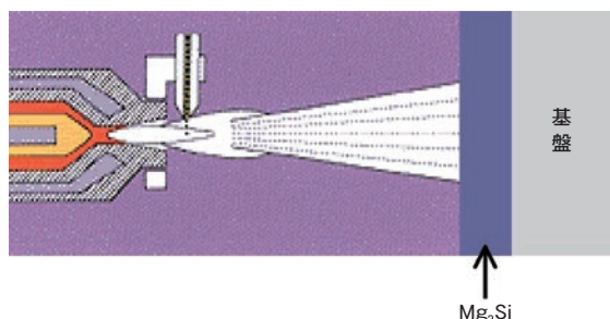
図9 粉末フレイム溶射の模式図 Fig.9 Schematic of powder flame spraying
