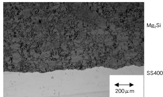
図11 溶射被膜の断面 Fig.11 Optical microstructure of coating
