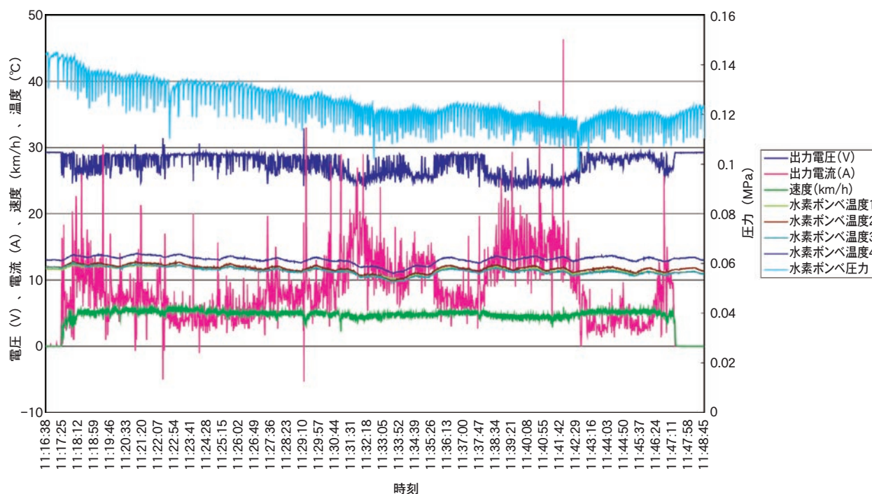
図9 燃料電池車いすの走行試験結果 Fig.9 The running test result of fuel cell wheelchair
