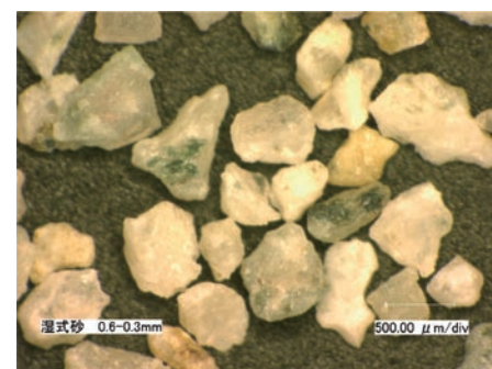
図6 既設湿式砕砂 (0.6~0.3mm)
